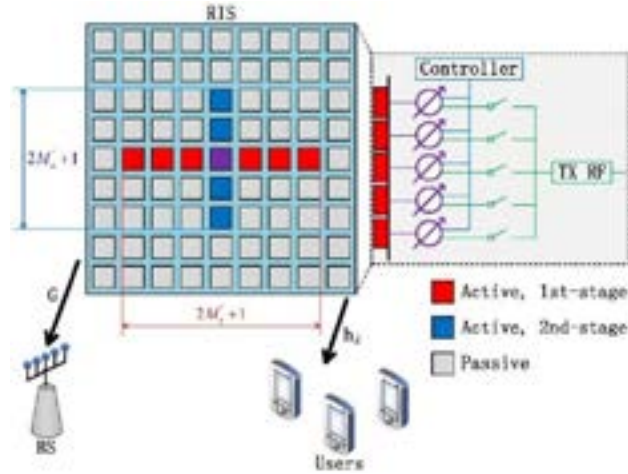
Fig. 5.11 RIS architecture transmitting pilots using one RF-chain.
