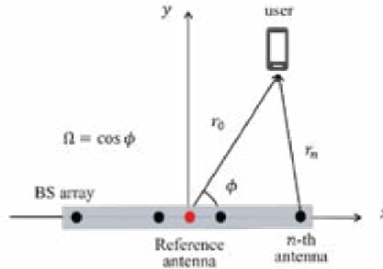
Fig. 4.28 System model
