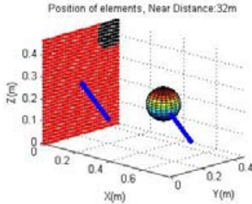
Fig. 4.11 The position of antenna array and PEC sphere as well as the incident wave vector H-POL V-POL
