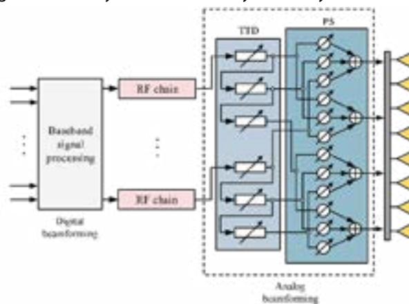
Fig. 5.15 Serially-Connected Delay-Phase Hybrid Beamforming
