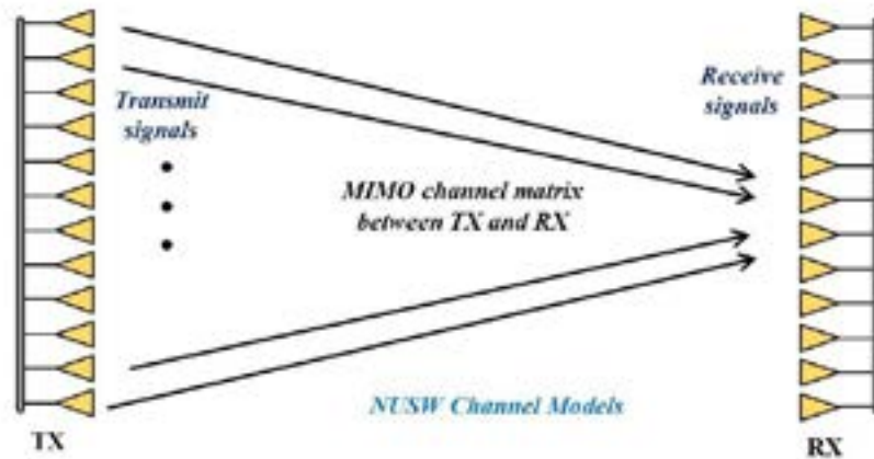
Fig. 4.20 NUSW channel model for spatially discrete antennas
