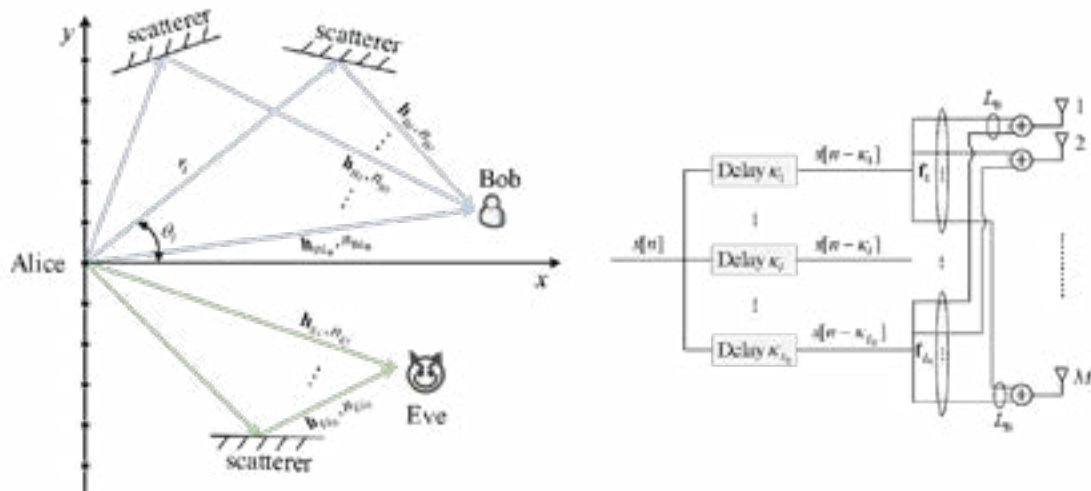
(a) A near-field secure communication system (b) Transmitter architecture for DAM Fig. 6.51 Near-field secure wireless communication with DAM.
