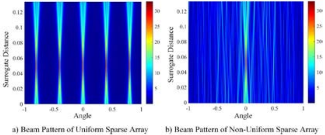
Fig. 5.24 Comparison of uniform and non-uniform sparse arrays in terms of the beam pattern. Moreover, it can be seen in Fig. 5.25 that the proposed non-uniform sparse array offers significant advantages in terms of supporting a higher number of users and improving data rate performance compared to existing uniform half-wavelength-spaced arrays and uniform circular arrays. Therefore, employing the beamforming scheme with non-uniform sparse arrays presents new possibilities for developing efficient near-field multi-user communication systems.
