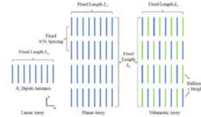
Fig. 3.35 Three types of near-field holographic array topologies
