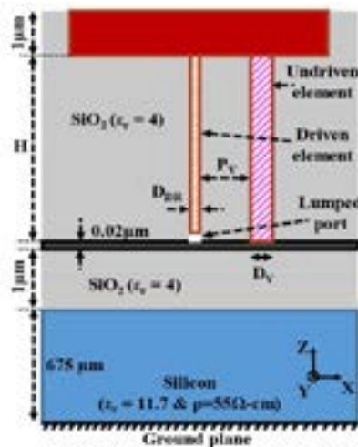
Fig. 6.63 Cross-section of the on-chip top-hat antenna [437].
