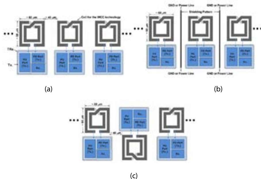
Fig. 6.65 (a)Typical coil array structure, (b)Coil array structure with a shielding pattern, (c)Proposed zigzag-shaped coil array for wireless chip-to-chip communication.
