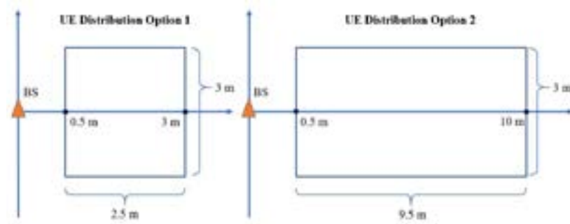
Fig. 5.45 UE distribution
