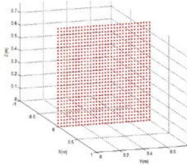
Fig. 4.6 The deployment of large antenna array (6GHz, 1024elements)
